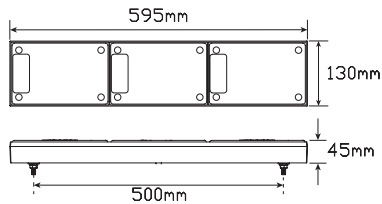
Part No. J3B3B
